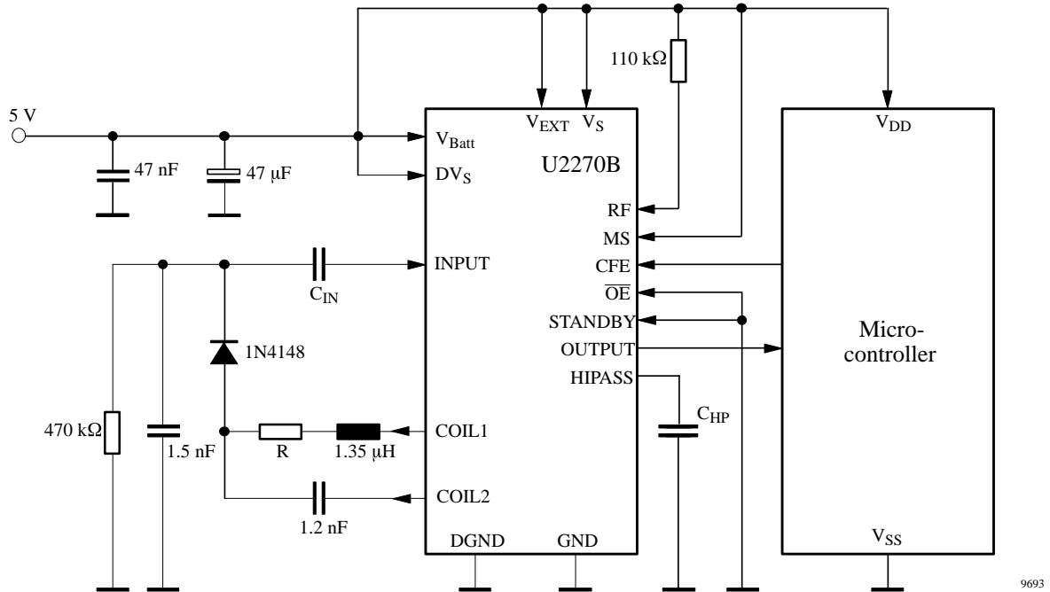
Figure 14. Application circuit
